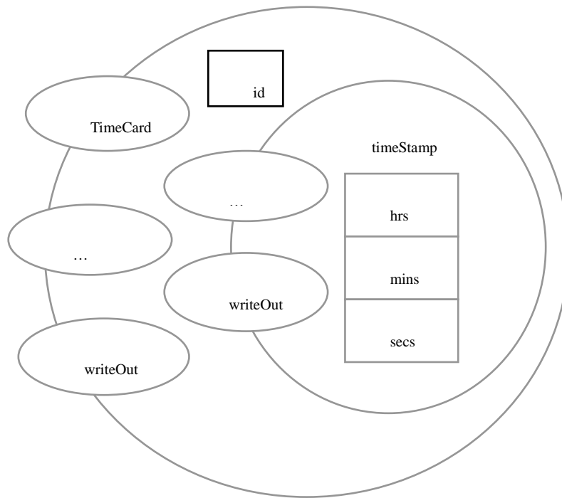
Fig. 13.3 The diagram of the nested class, TimeCard .
